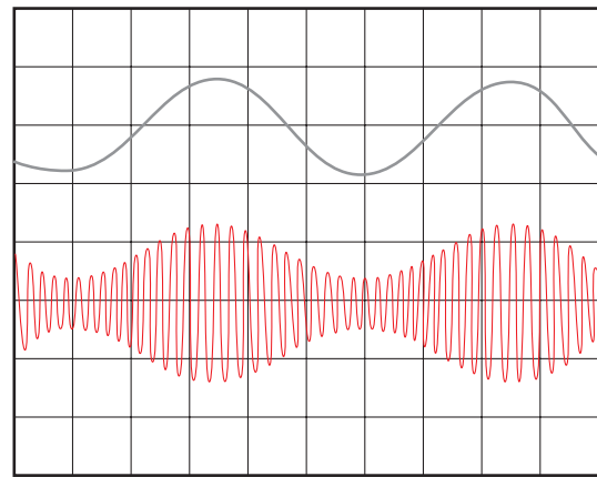
External source: V_{in} = 0.5 V_{rms} = 0.7 V_p , 1 kHz, 1 V/cm HM 8131-2: V_o = 10 V_{pp} , 20 kHz, 5 V/cm, 100 % modulation selected
