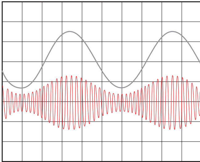
External source: V_{in} = 1.4 V_p , 1 kHz, 1 V/cm HM8131-2: V_o = 10 V_{pp} , 20 kHz, 5 V/cm, 50 % modulation selected
