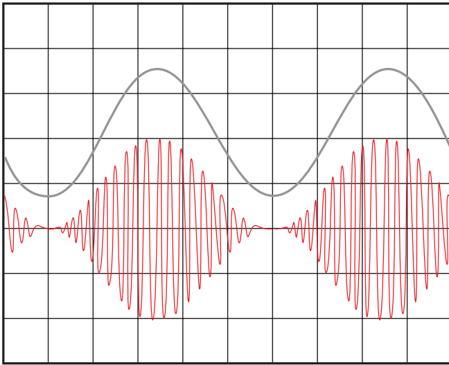
External source: V_{in} = 1.4 V_p , 1 kHz, 1 V/cm HM 8131-2: V_o = 10 V_{pp} , 20 kHz, 5 V/cm, 100 % modulation selected
