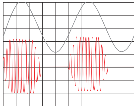
External source: V_{in} = 4.00 V_p , 1 kHz, 2 V/cm HM 8131-2: V_o = 10 V_p , 20 kHz, 5 V/cm, 35 % modulation selected → generator overmodulated
