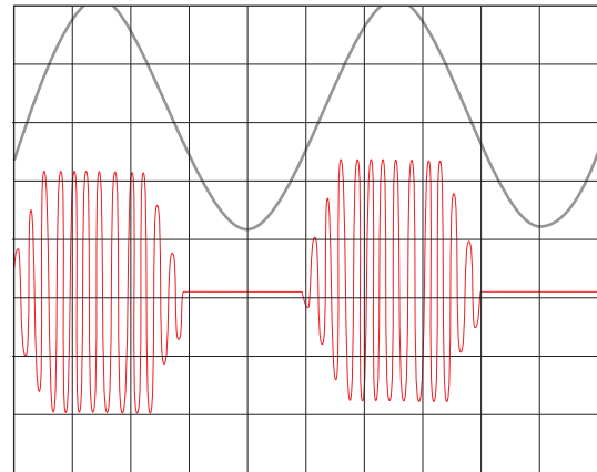
External source: V_{in} = 4.00 V_p , 1 kHz, 2 V/cm HM8131-2: V_o = 10 V_p , 20 kHz, 5 V/cm, 100 % modulation selected → generator overmodulated
